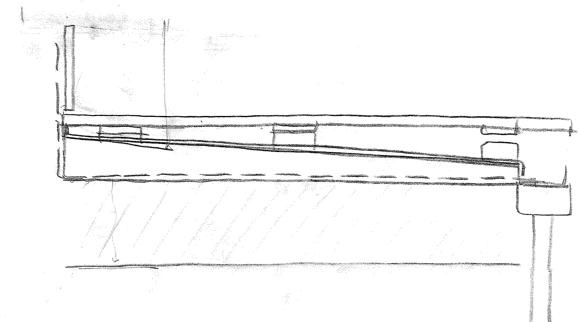
Waterproofing to slab roof showing concrete tiles on 'chairs'
