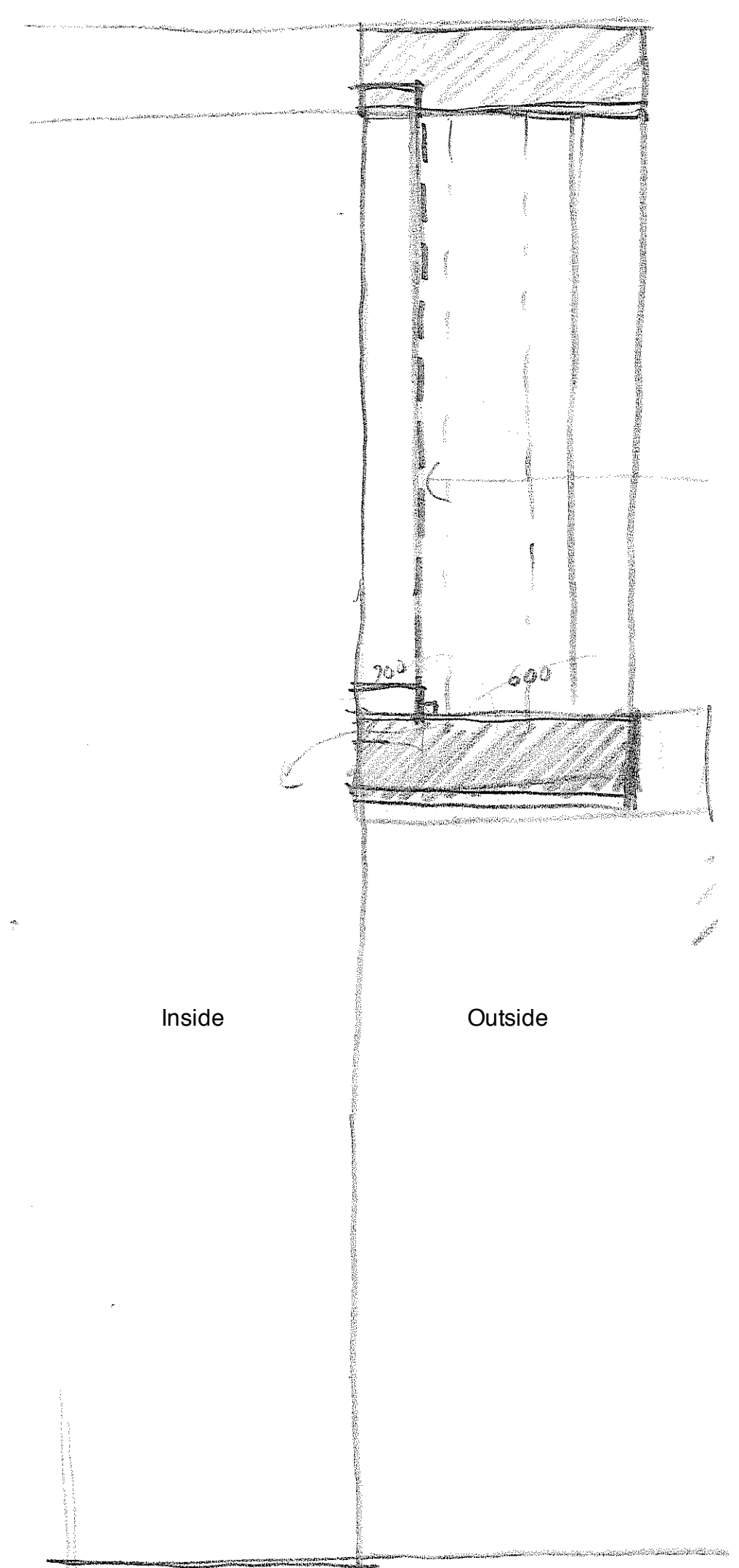
high level glazing / timber screen to living area section detail
