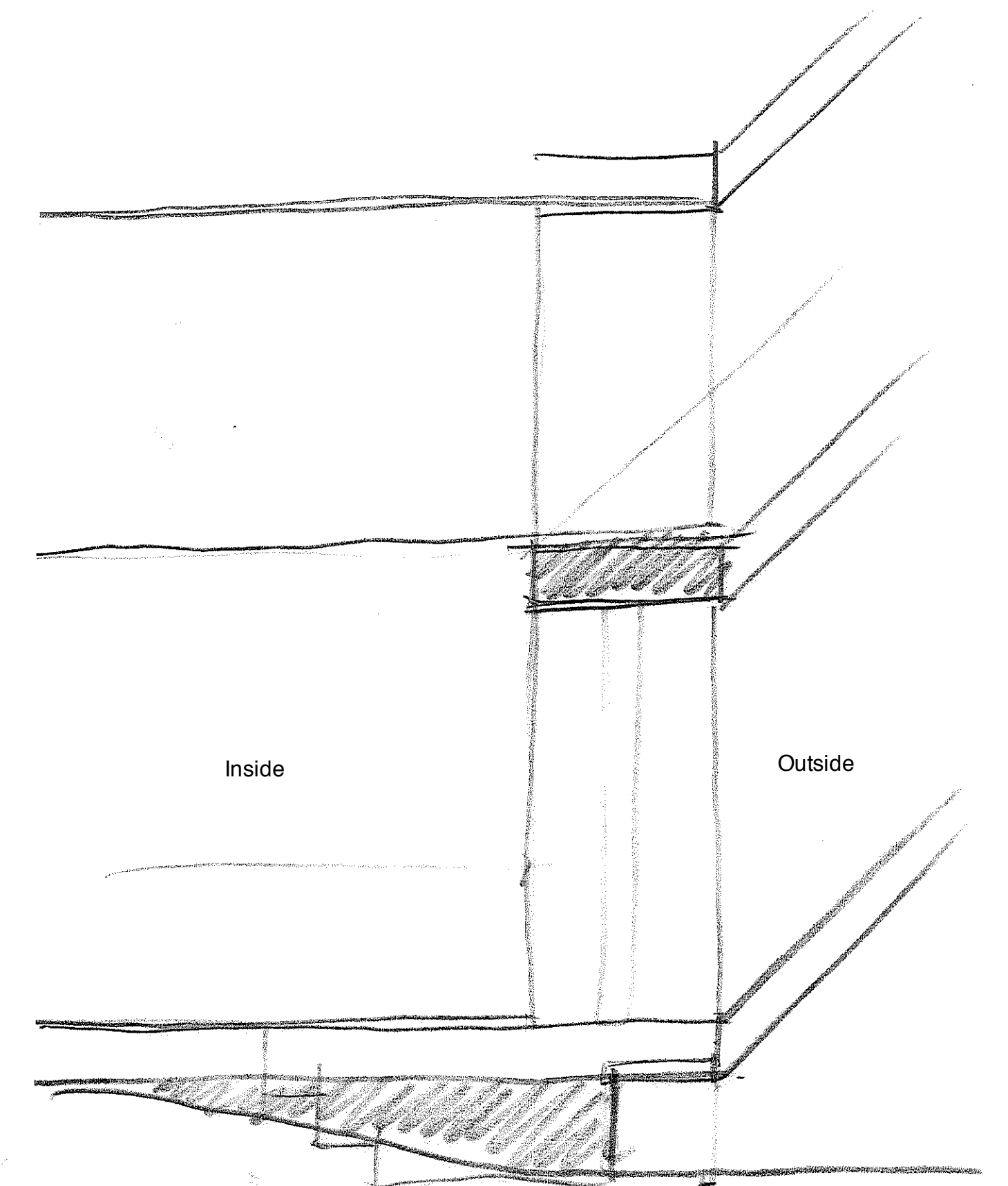
Flat slab concept - shown floating above receding natural ground line
